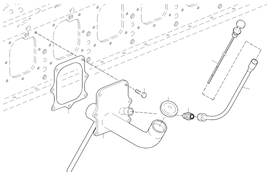
OIL FILLER NECK UPC.06G04 1429
