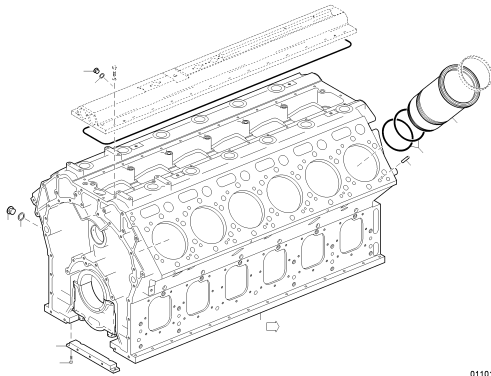
CRANKCASE UPC.06A01 0928
