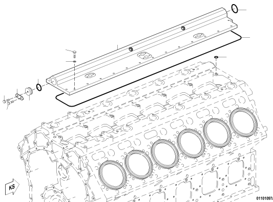
TOP VALLEY COVER SINGLE PASSAGE INDUSTRI UPC.06A01D0014
