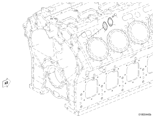
CVR CYL INSPECTION PORT 12V S4000 UPC.06A01B0231
